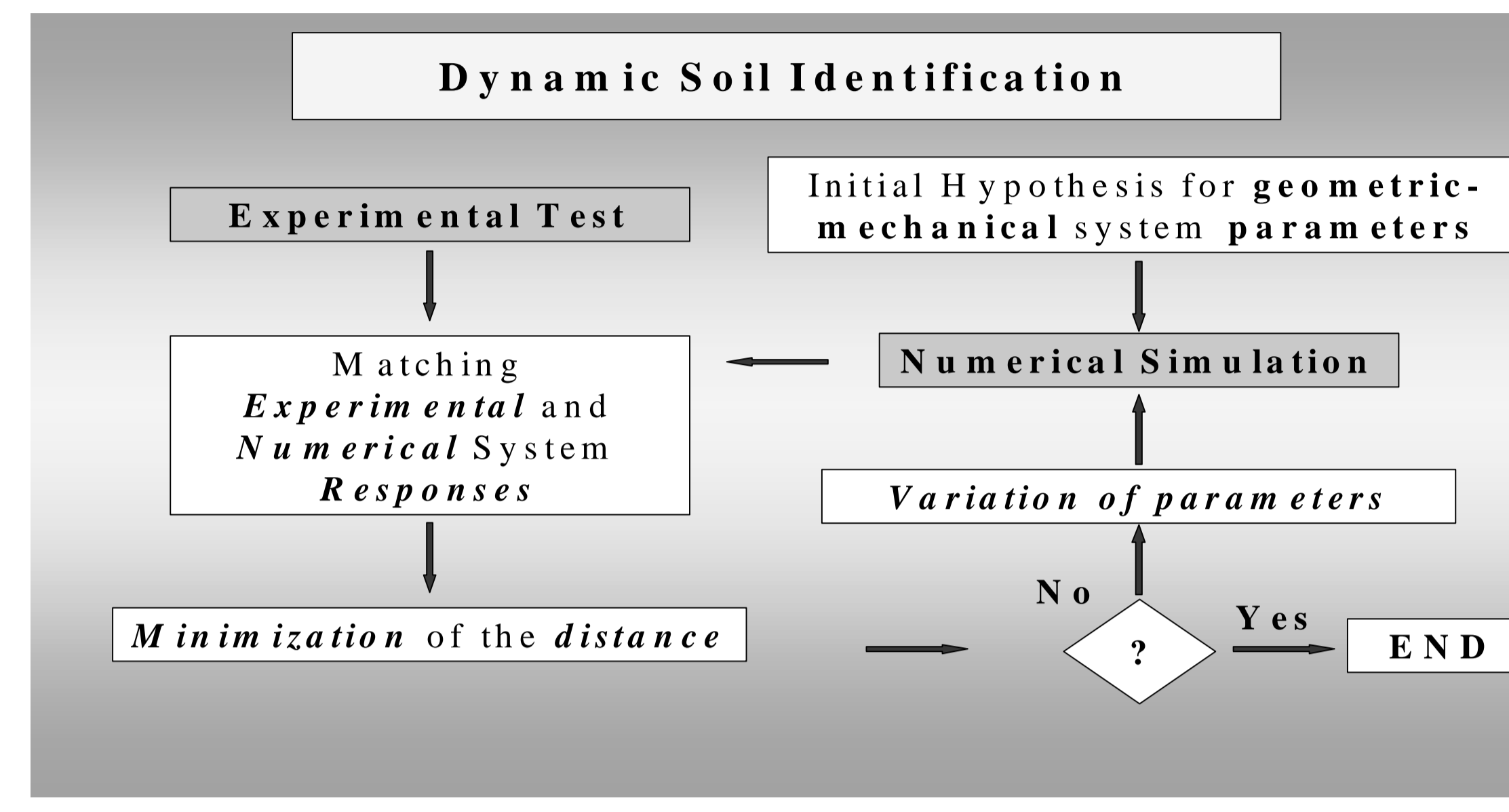
2) Inversion Procedure: Experimental Test + Numerical Simulation + Optimization Problem
